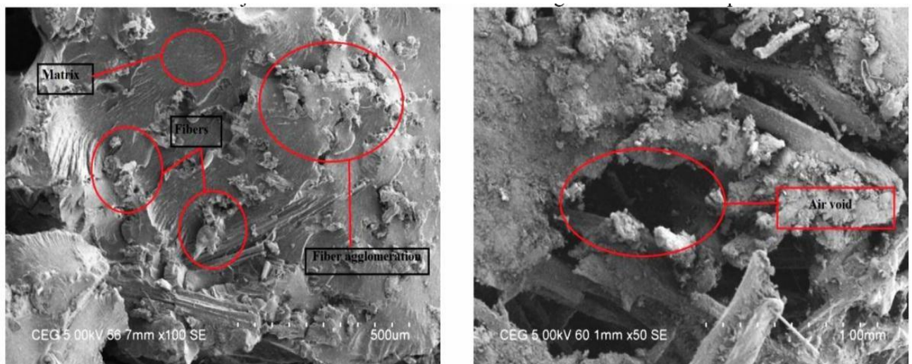
Figure 8. (a) 500µm magnification SEM image for jute epoxy composite; (b) 1mm magnification SEM image for jute epoxy composite
