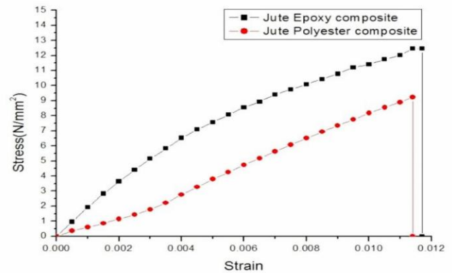
Figure. 5. Tensile test stress - strain curves for 5 % NaOH treated jute reinforced composites
