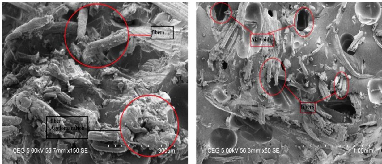
Figure 9. (a) 300 μm magnification SEM image for jute polyester composite; (b) 1 mm magnification SEM image for jute polyester composite
