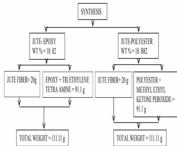
Figure 2. Synthesis of jute fiber reinforced composites in terms of weight percentage.
