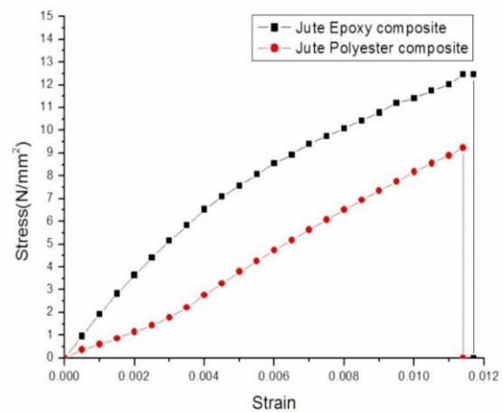
Figure 5. Tensile test stress - strain curves for 5 % NaOH treated jute reinforced composites
